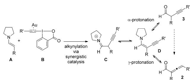
Scheme 2. Proposed synergistic strategy for the \alpha -vinylidenation of aldehydes.
